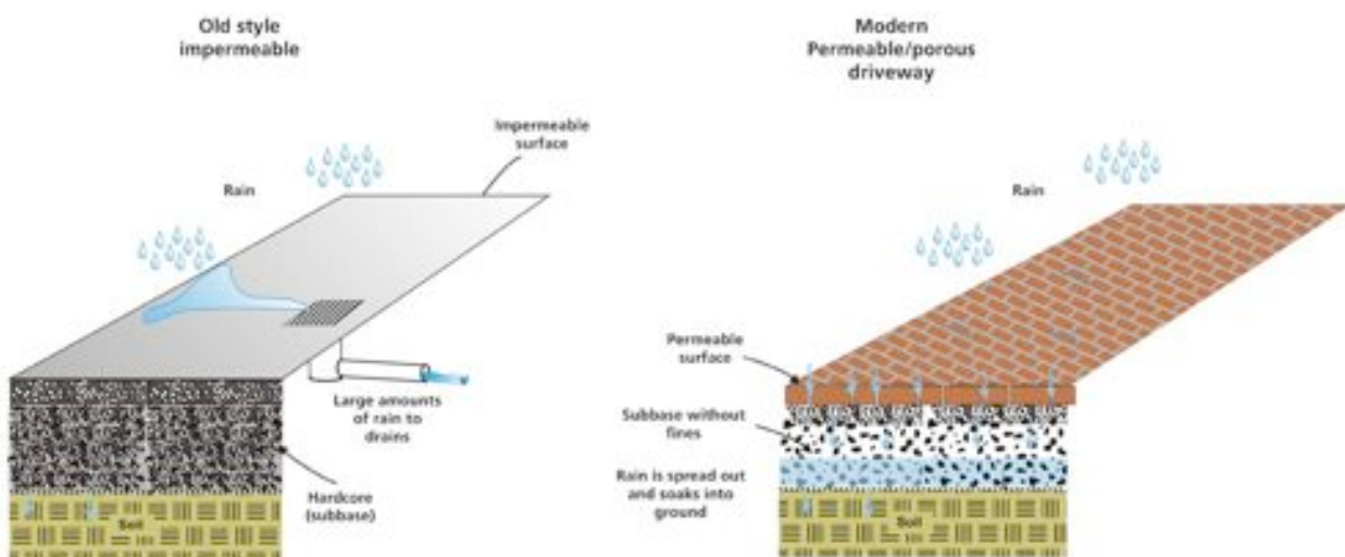
Permeable modern vs old style impermeable driveways
